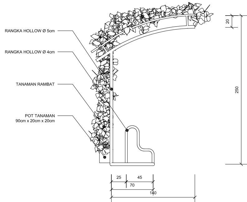
TAMPAK SAMPING
